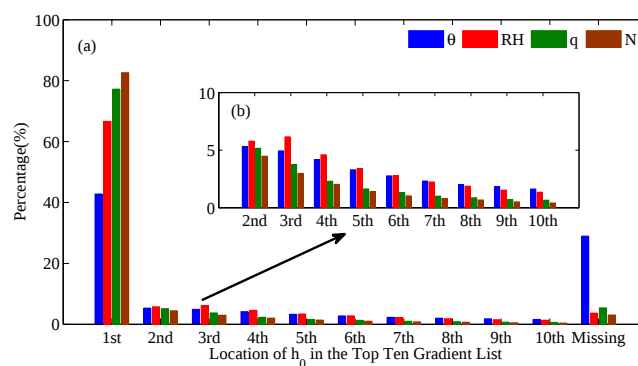
Figure 4. The statistical result of the consistency between h_0 ( h_0 which integrates the information of \theta , RH, q and N ) and the four existing methods at the 79 North America stations. Percentage in “1st” means the h_0 coincides with the existing method. The missing value means the case of the h_0 did not exist in the top 10 gradient lists for the specific variable and the h_0 is determined by the other three standards. The subgraph (b) shows a close-up view of the 2nd to 10th in (a).
